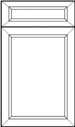
Gamma
